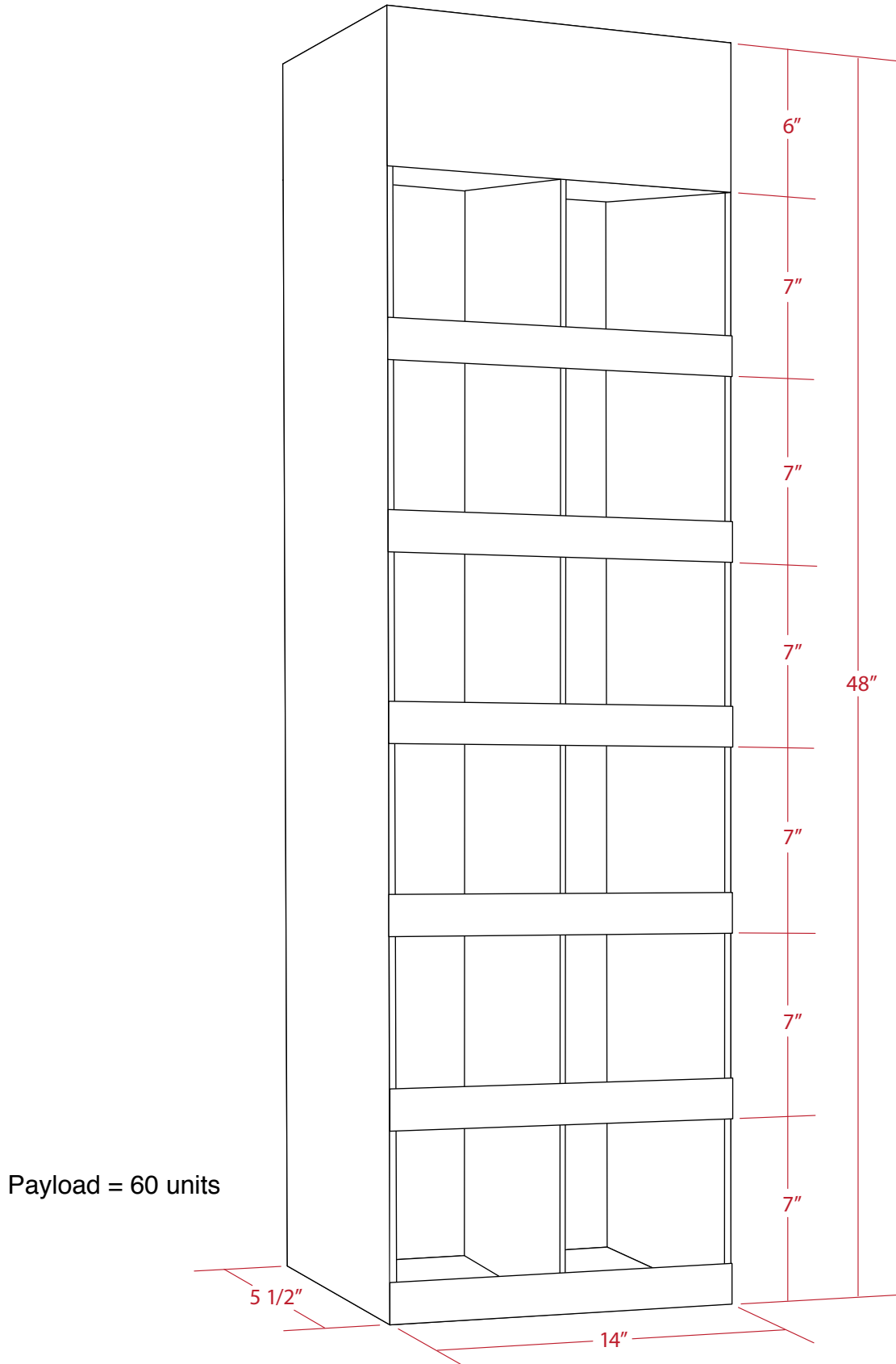
FirstAide | Sidekick Dimensions & Payload
